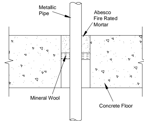
Metallic Pipe through Concrete Floor
